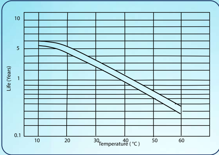
Float life vs Temperature
