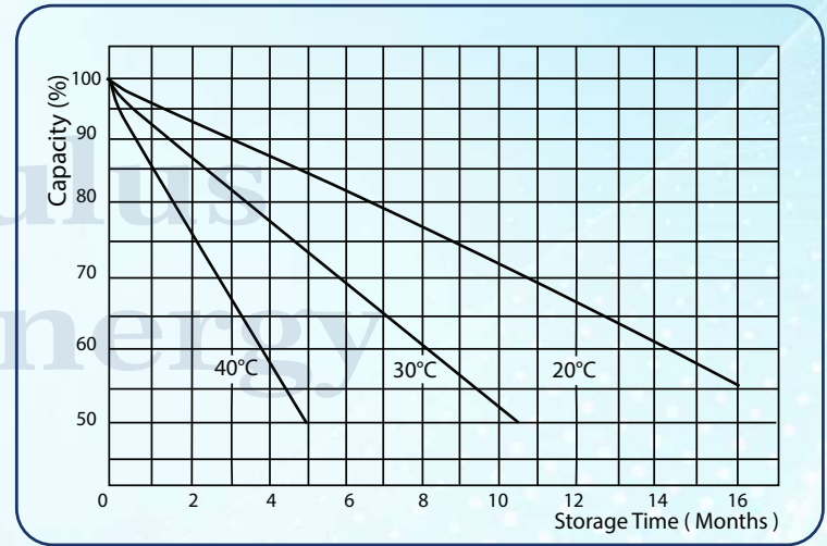
Self-discharge Characteristics
